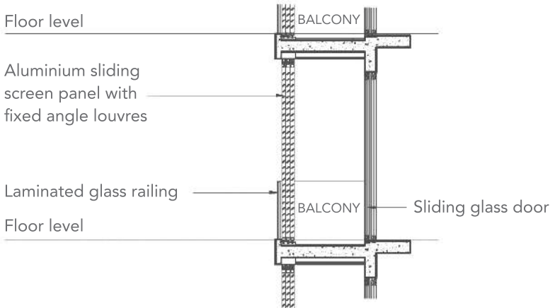
TYPICAL RETRACTABLE BALCONY SCREEN - SECTION
